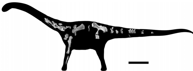
FIGURE 3. Silhouette reconstruction of Rukwatitan biseptus to illustrate those portions of the skeleton recovered from locality RRBP 2007-02 and included as part of the holotype. Scale bar equals 1 m.
